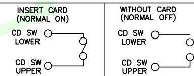
Circuit Diagram for Card Detect Switch
