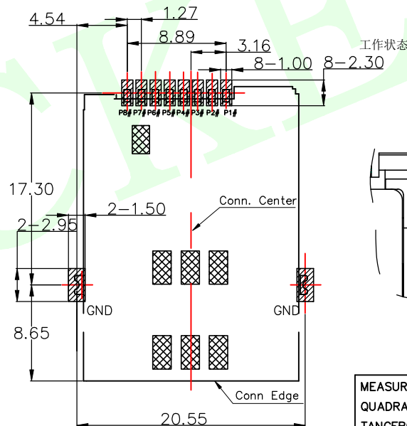
RECOMMENDED PCB LAYOUT(TOP VIEW) GENERAL TOLERANCES: \pm 0.05
