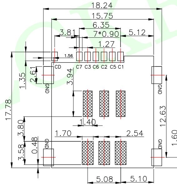
RECOMMENDED PCB LAYOUT GENERAL TOLERANCE ±0.05
