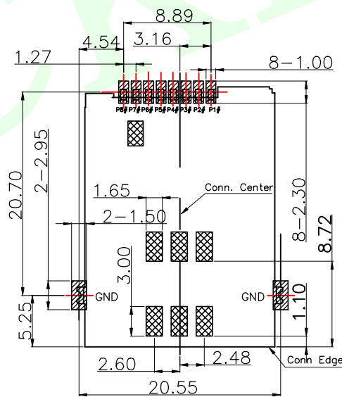
RECOMMENDED PCB LAYOUT(TOP VIEW) GENERAL TOLERANCES:±0.05
