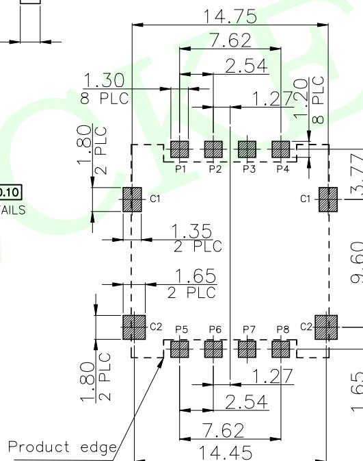
RECOMMENDED PCB LAYOUT(TOP VIEW) GENERAL TOLERANCES: ±0.05
