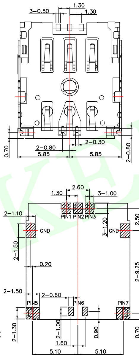
PCB LAYORT (TOP VIEW) TOLERANCE: ±0.05
